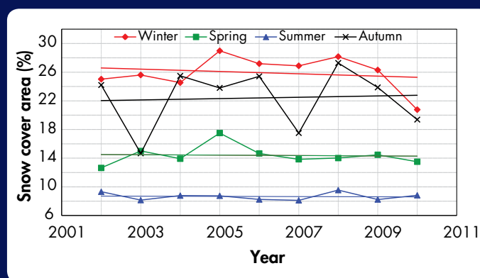
Figure 26: Seasonal variation in SCA in the HKH region, 2002–2010
