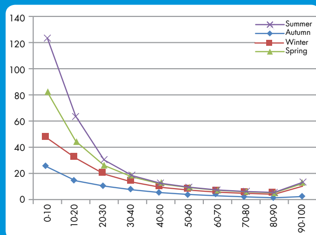
Figure 27: SCA for classes of snow occurrence in different seasons (%)
