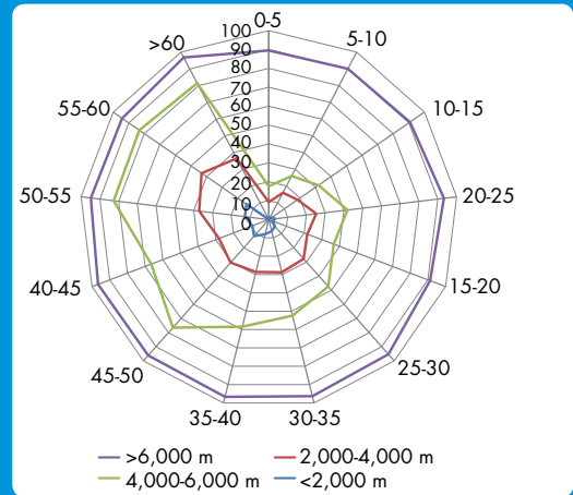
Figure 19: Distribution of snow cover in relation to elevation and slope
