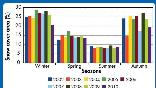
Figure 25: Seasonal SCA, 2002–2010
