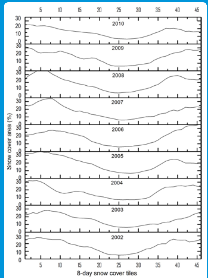
Figure 24: Intra-annual variations in snow cover area in the HKH, 2002–2010
